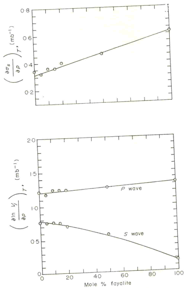
FIG. 2. Pressure coefficient of P and S wave velocities and pressure derivative of Poisson's ratio as a function of (Fe/Mg) ratio in olivine.
